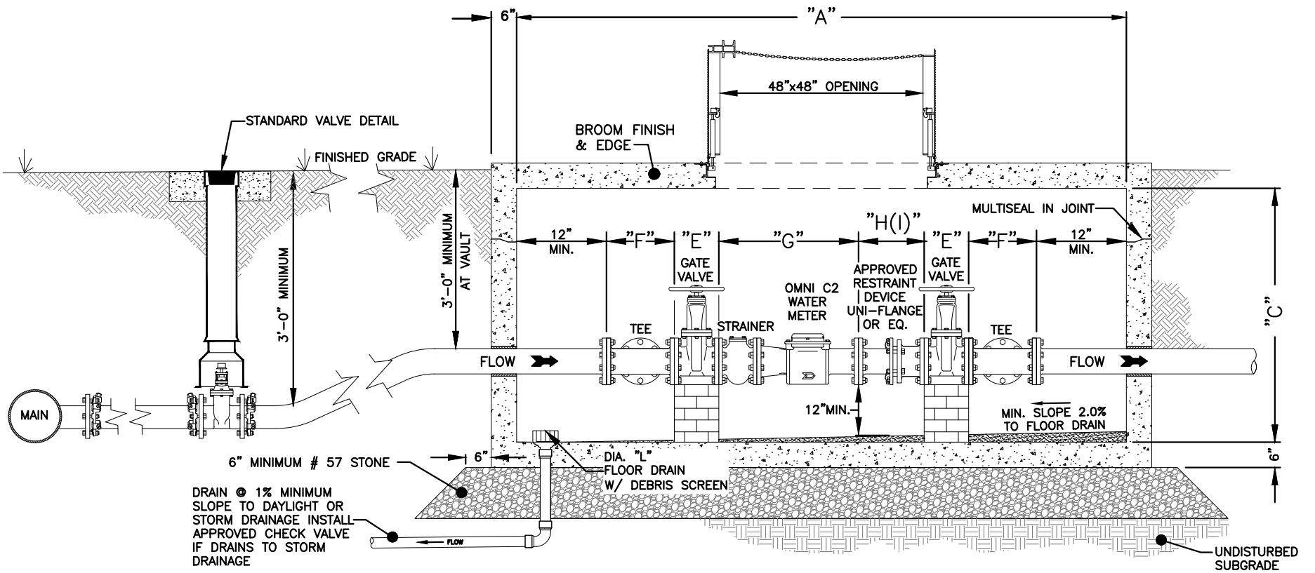
SECTION VIEW NOT TO SCALE
