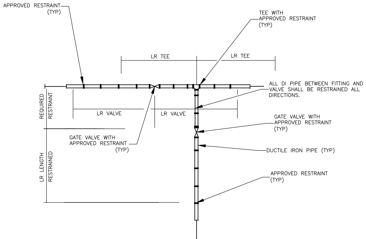
RESTRAINED JOINT DETAIL FOR TYPICAL TEE INTERSECTION 4 WAY INTERSECTION SIMILARLY RESTRAINED
