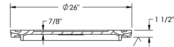
MANHOLE COVER
