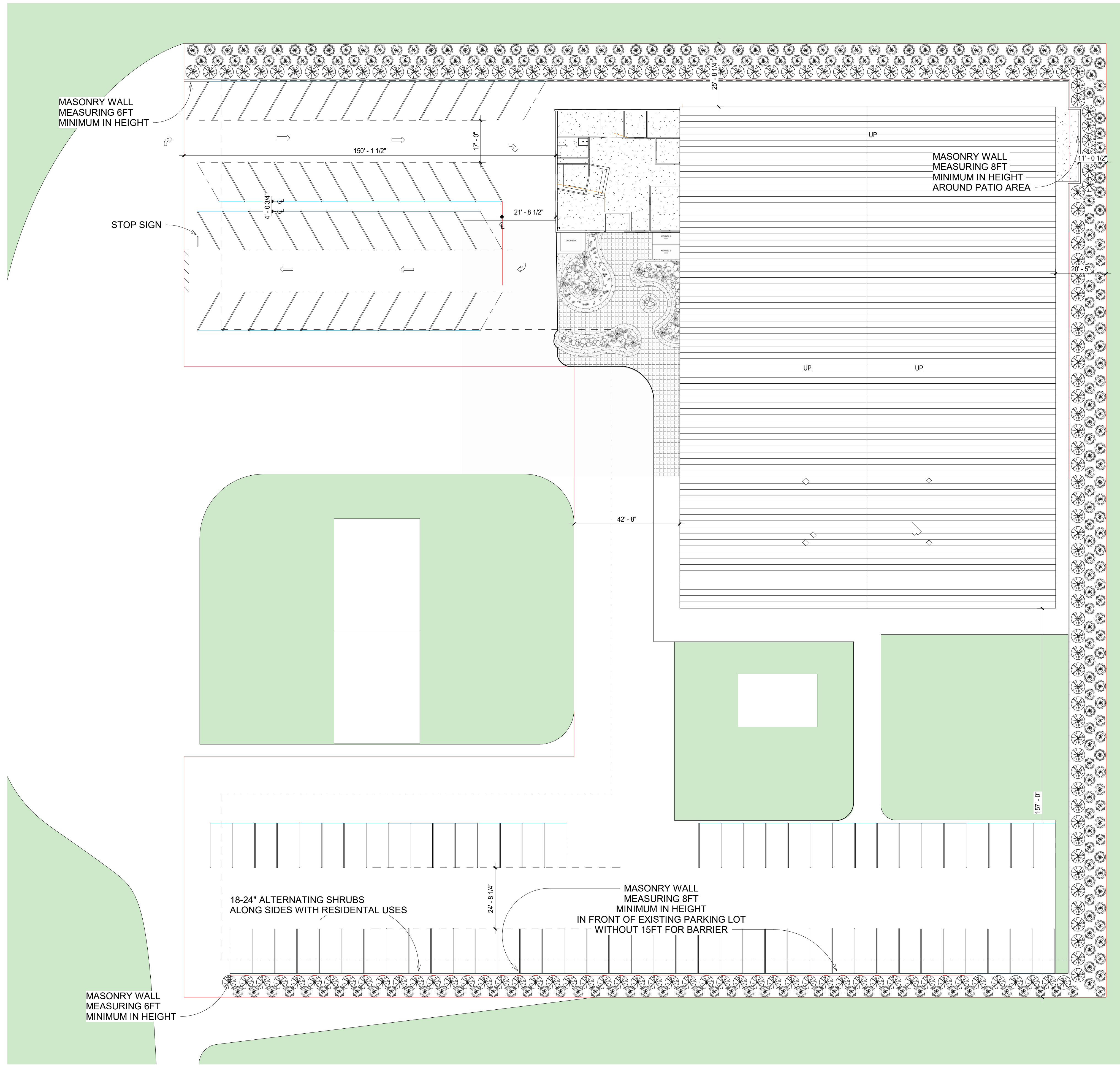
1 SITE PLAN SP101/ 3/64" = 1'-0"
